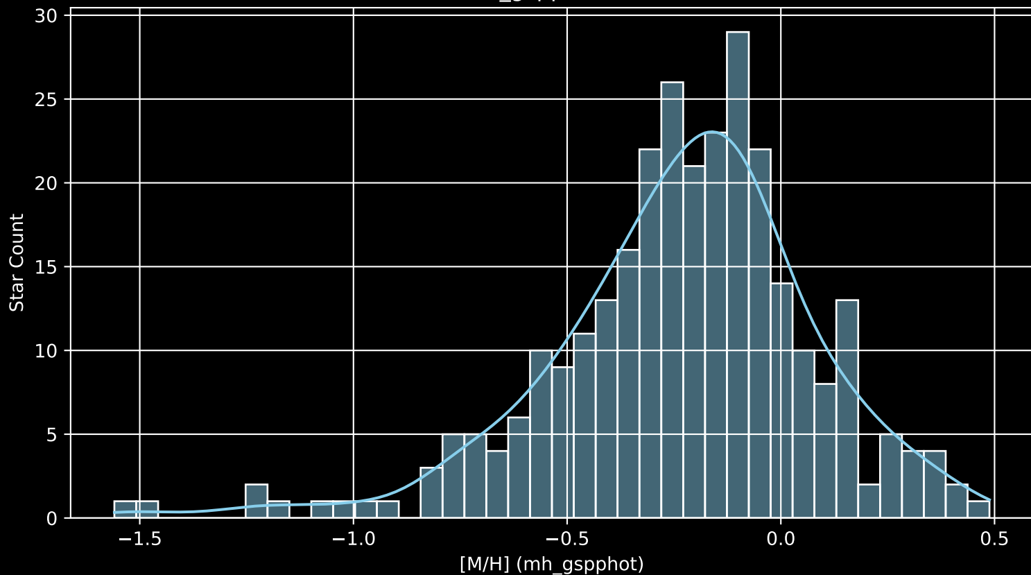
APOGEE DR17 Field: [094-43_MGA [M/H] (mh_gspphot) (n= 297)
