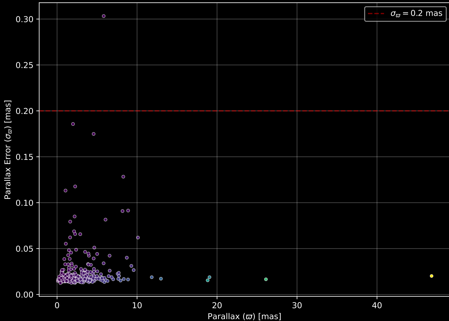
APOGEE DR17 Field: [094-43_MGA] Parallax Quality (n= 300)
