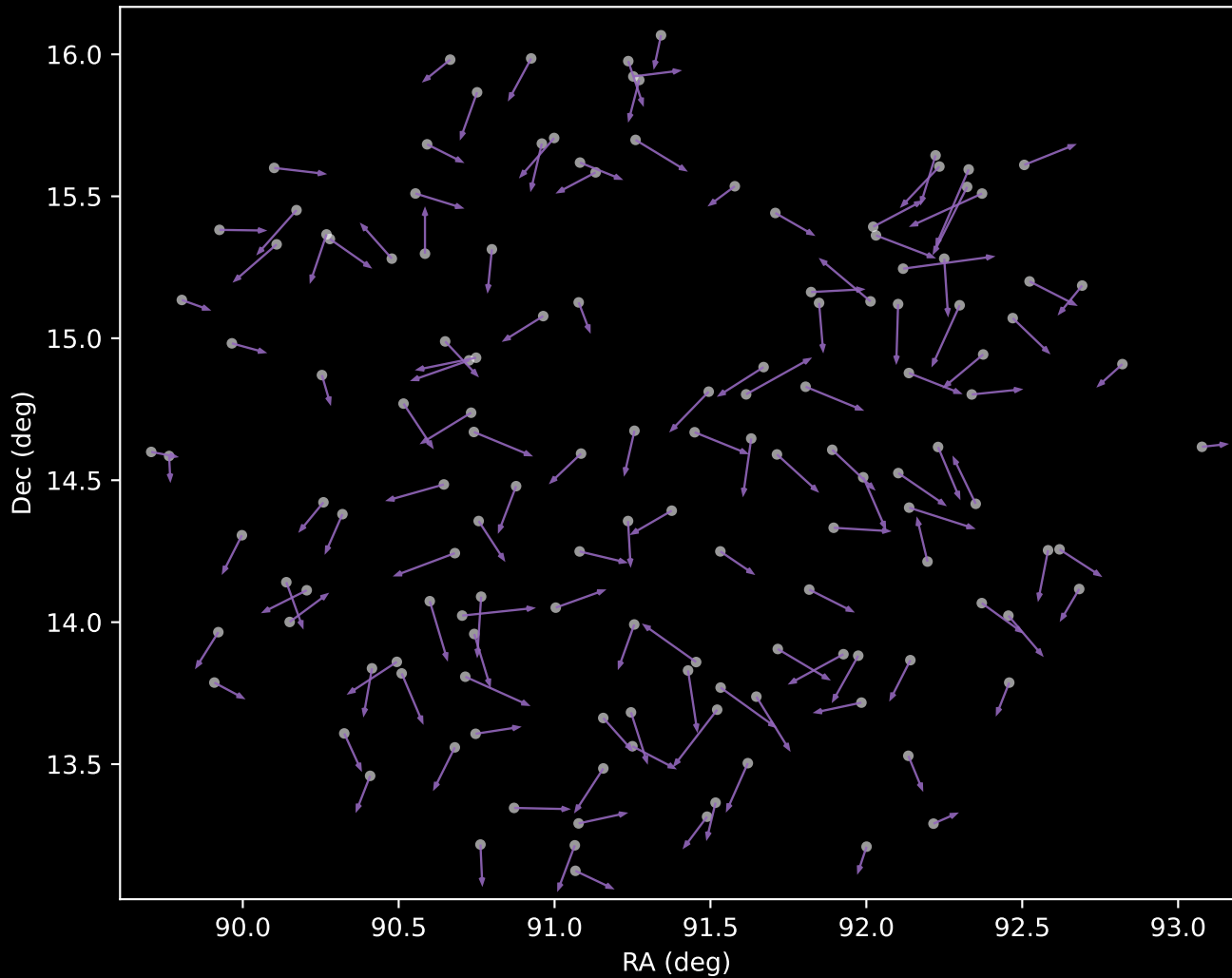
APOGEE DR17 Cluster 8 Proper Motion Vectors (n=140)
