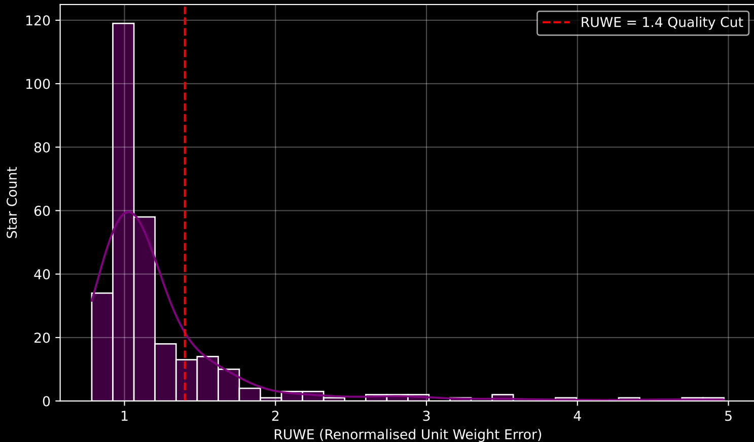
GAPOGEE DR17 Field [094-43_MGA] RUWE Distribution (n= 291)
