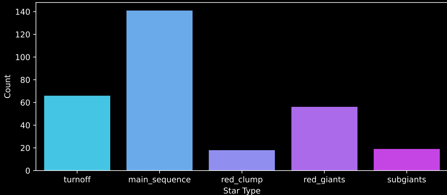
APOGEE DR17 Field: [094-43_MGA] Count plot of Star Type
