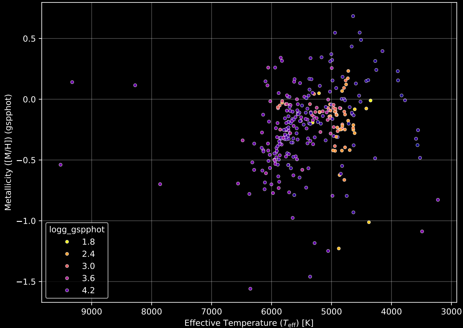
APOGEE DR17 Field: [094-43_MGA] Stellar Population Parameters (n= 300)
