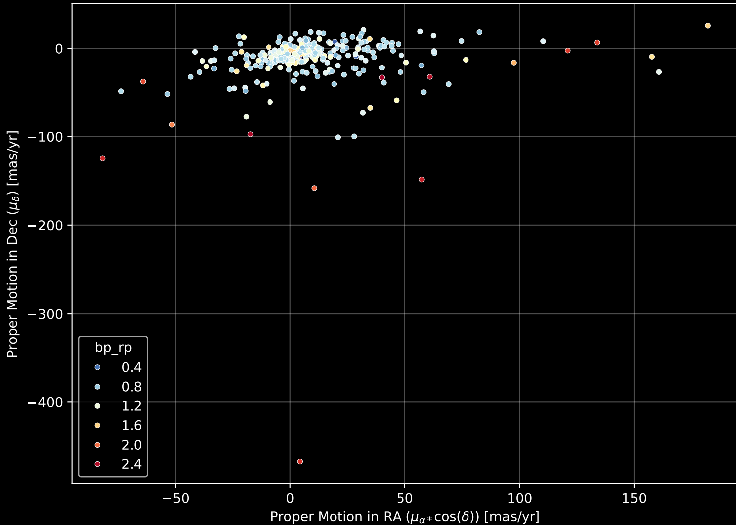
APOGEE DR17 Field: [094-43_MGA] Proper Motion Diagram (n= 300)
